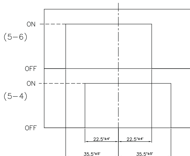
SWITCH SEQUENCE
